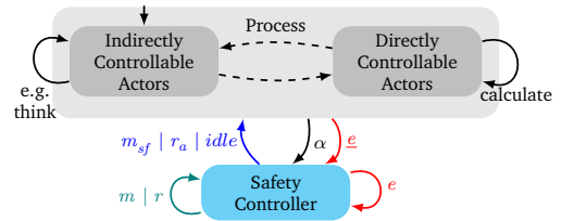
Figure 5: Execution from the viewpoint of the safety controller. The execution is coordinated by passing a single token between two groups of actors (dashed arcs) performing actions in the process. The controller can perform an update or issue control inputs to the process after every atomic event occurring in the process.
