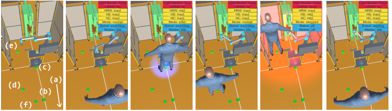
(a) System configuration for testing, with the operator's path highlighted by numbered waypoints. (b) Initial state. The operator waits in front of the workbench while the cobot moves to retrieve a work piece. (c) The controller issues mitigations as the operator and cobot simultaneously reach for the workbench ( HRW ). (d) The operator leaves the workbench while the cobot in response to the operator approaching the spot welder during operation ( HS and HC ). (e) The controller issues a stop in response to the operator approaching the spot welder during operation ( HS and HC ). (f) Welding resumes after operator leaves the work cell. The notification to leave the cell is deactivated.
